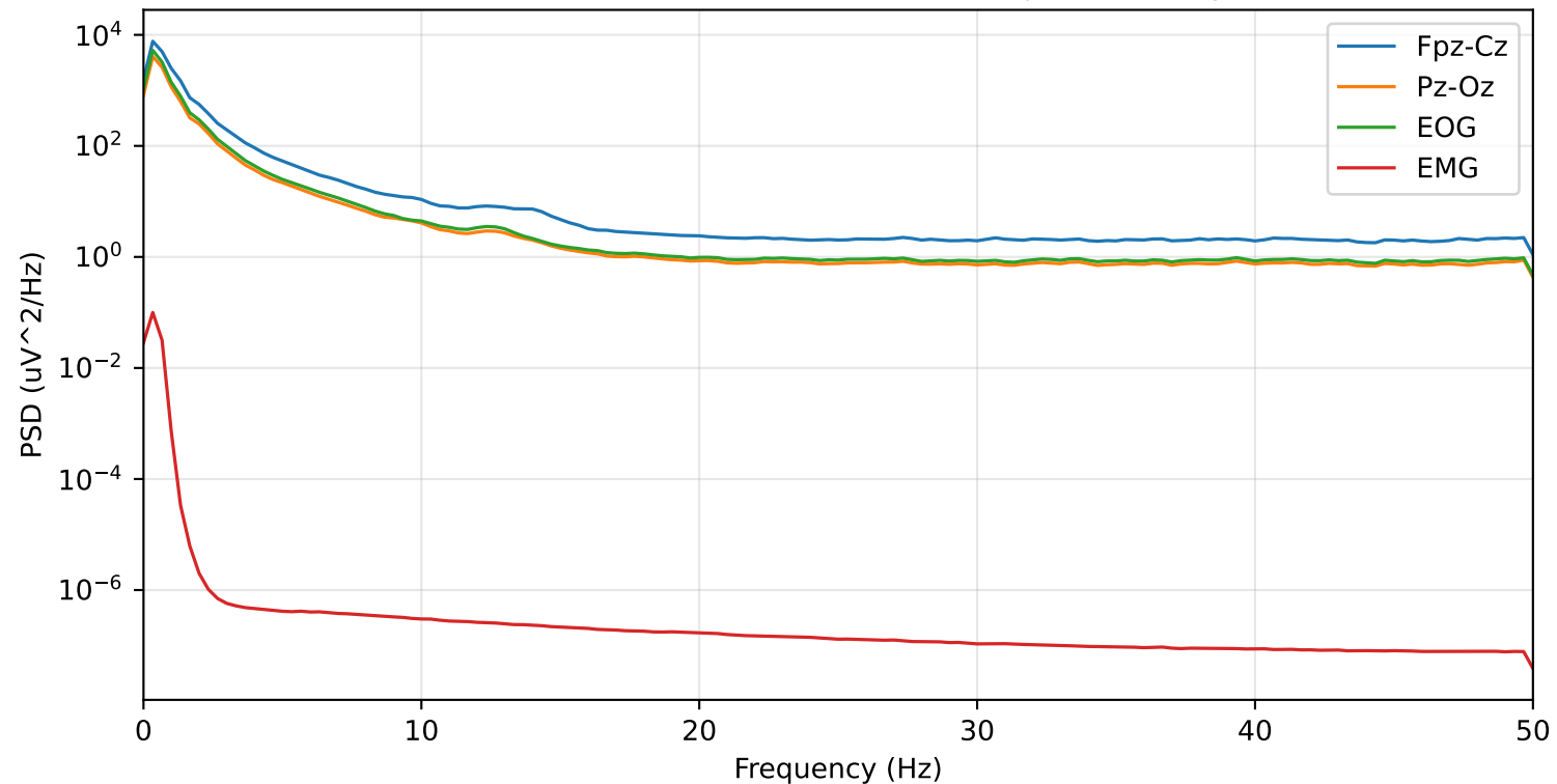
Mean PSD of the four PSG channels (subject 6, all epochs)
